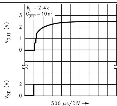
Figure 30. Turn-ON Waveform
